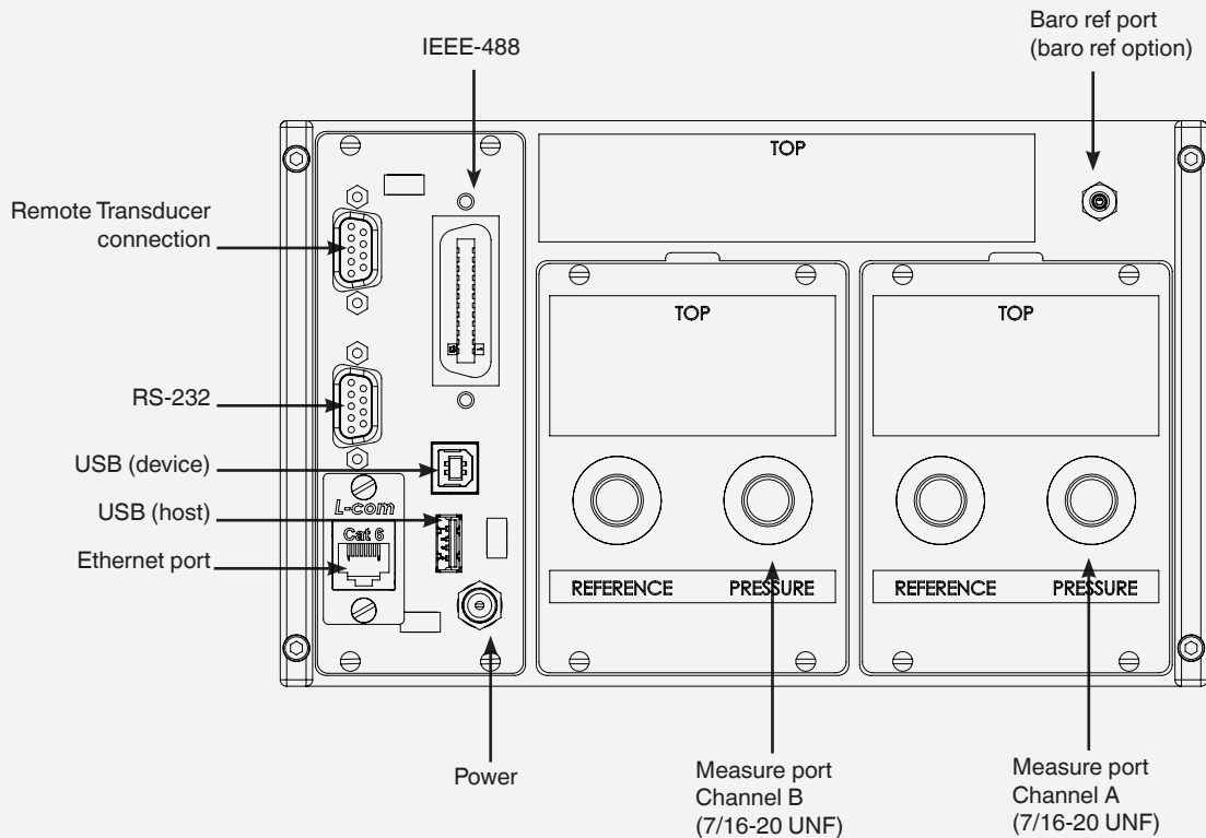
Rear Panel
