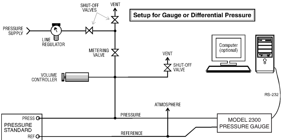
Figure 9.2 - Calibration Setup
