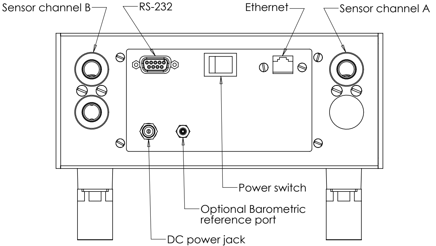
Electrical connections and pressure ports - rear view
