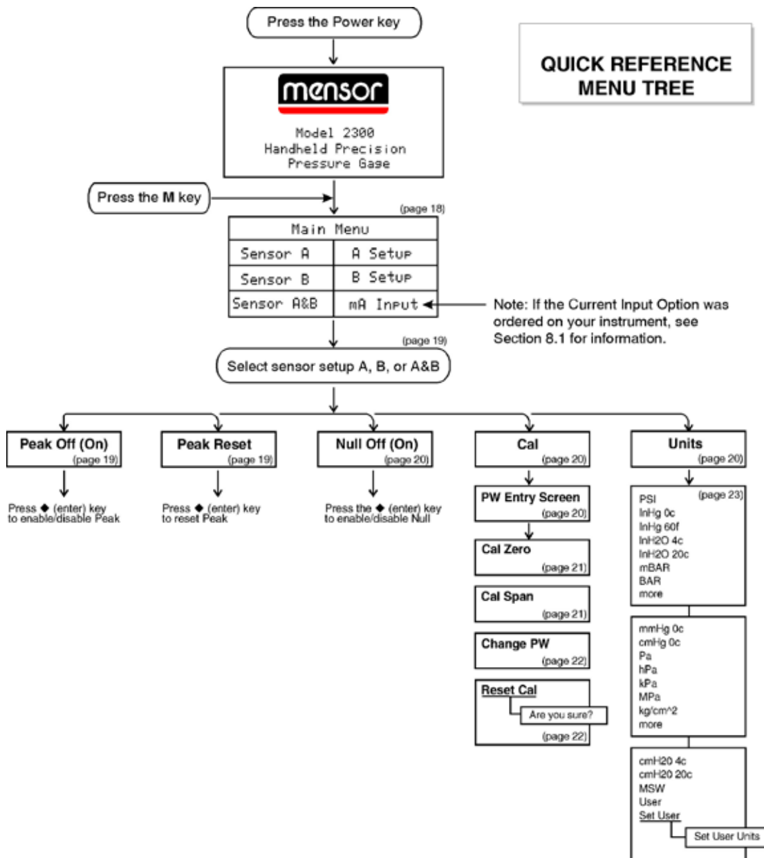
Figure 6.4 - DPG 2300 Menu Tree
