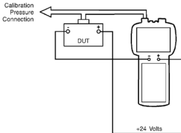
Figure 8.1.4b - Connections using DPG 2300 loop power
