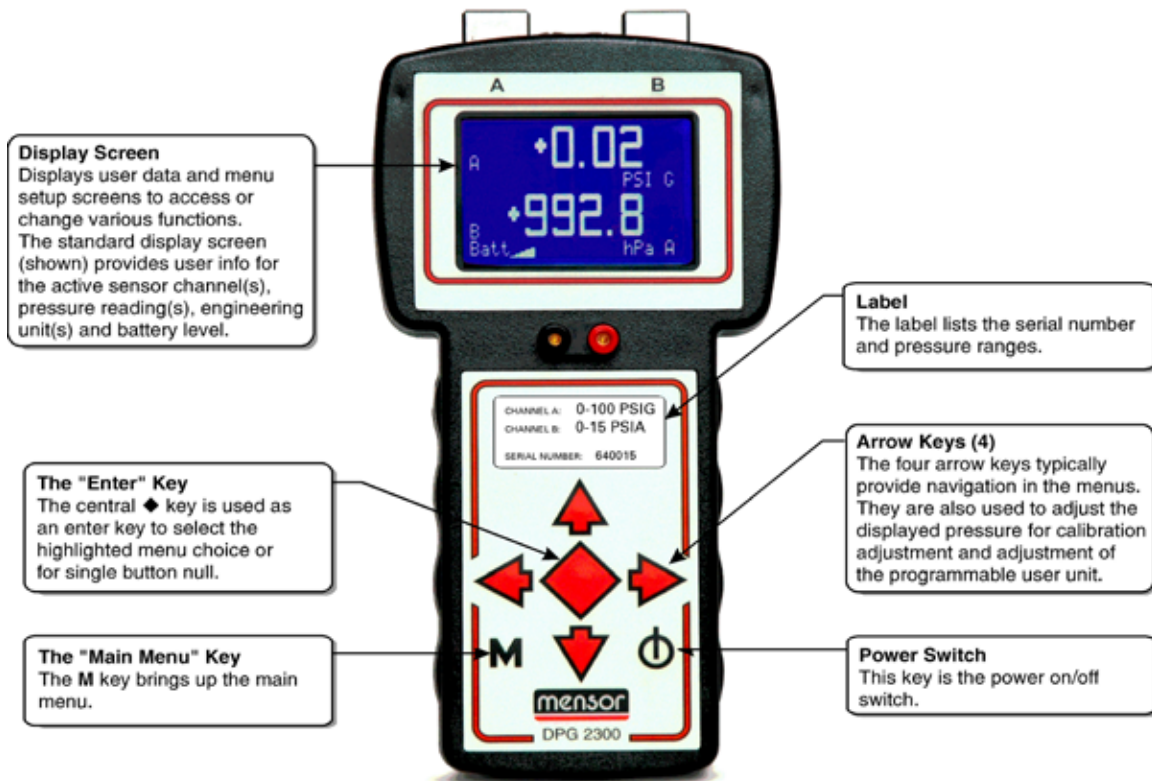
Figure 6.1 - Keypad and Display Features
