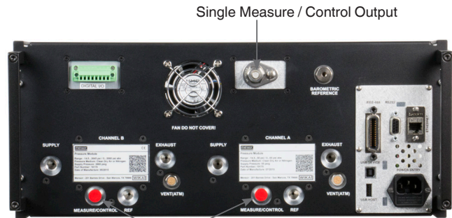
Plugged ports
