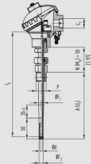
tapered thread
