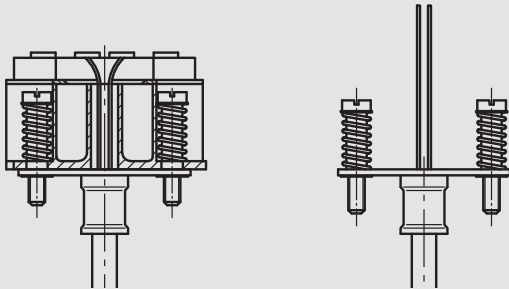
Measuring insert prepared for transmitter mounting
