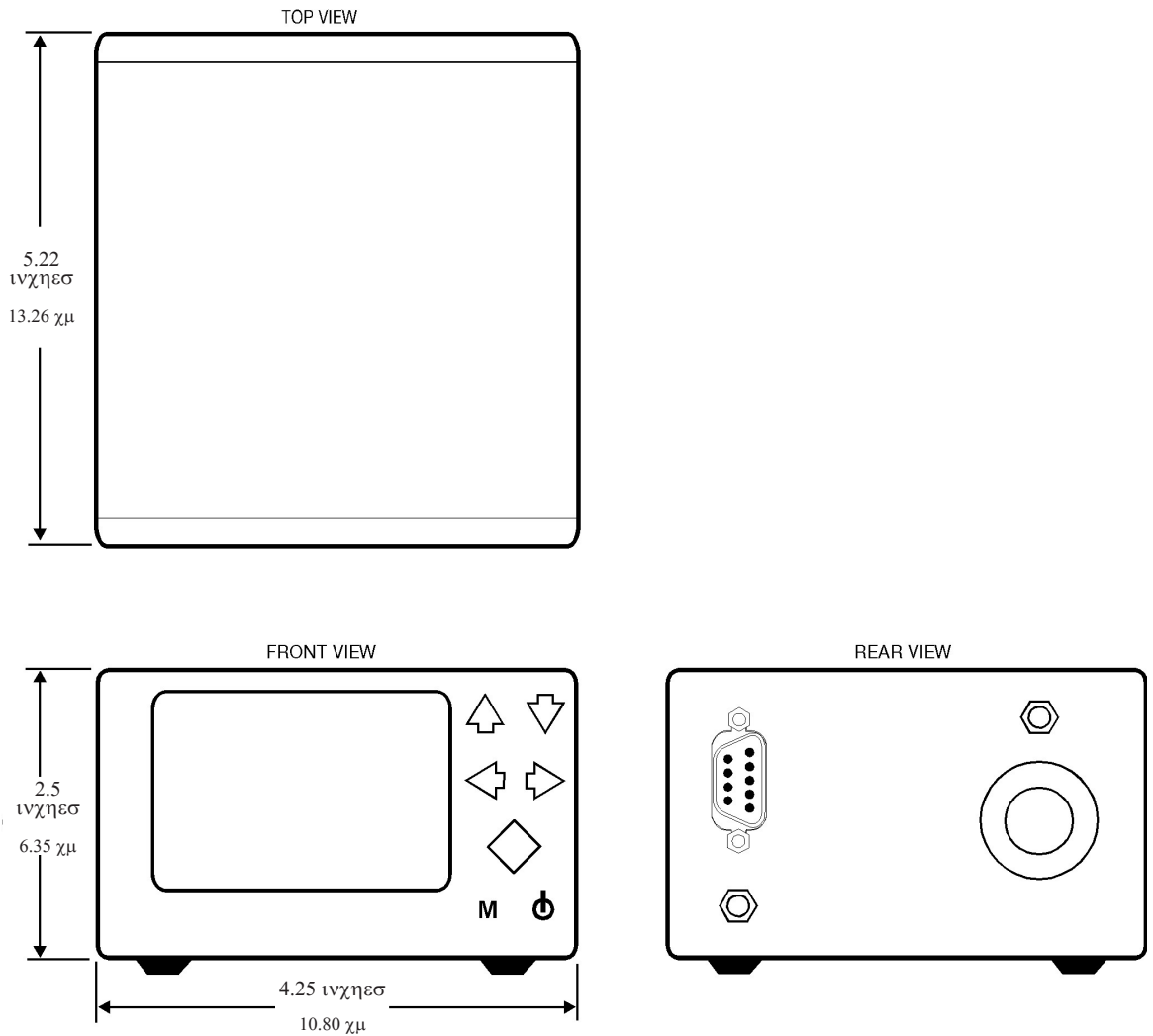
Figure 5.2 - Case Outline/Dimensions
