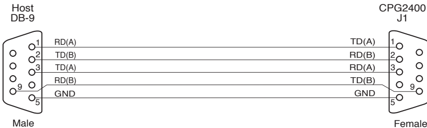
Figure 5.4b - RS-485 Hookup
