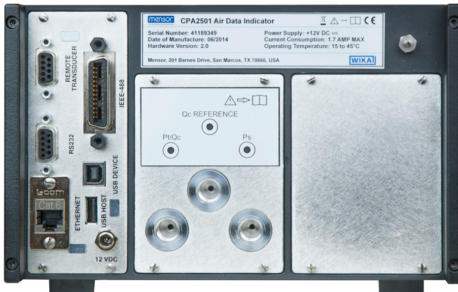
Figure 5.4 - Rear Panel
