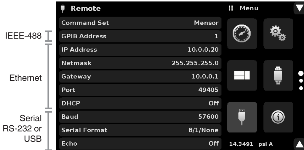
Figure 6.4.5 - Remote Application
