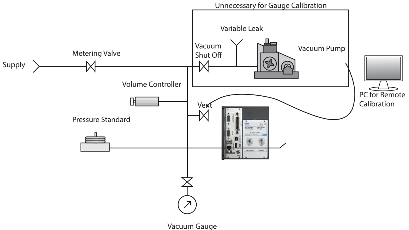
Figure 10.4 - Calibration Setup
