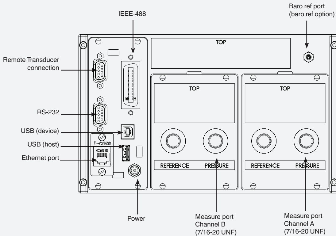
Rear Panel
