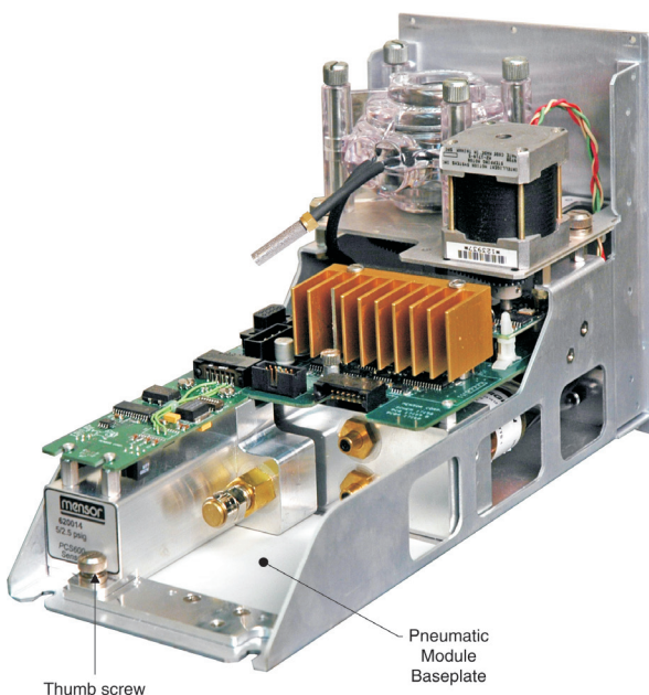
Figure 9.2.1B - Pneumatic Module, Pump Regulator
