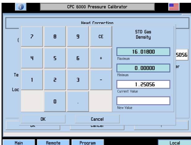
Figure 10.9C - Gas Density
