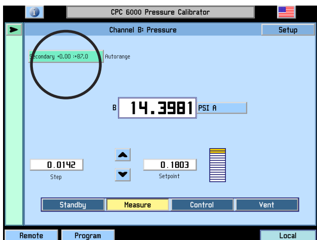
Figure 6.3.4A - [Turndown Label]
