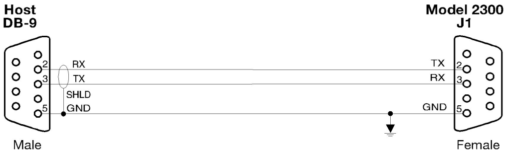
Figure 5.4a - RS-232 Hookup
