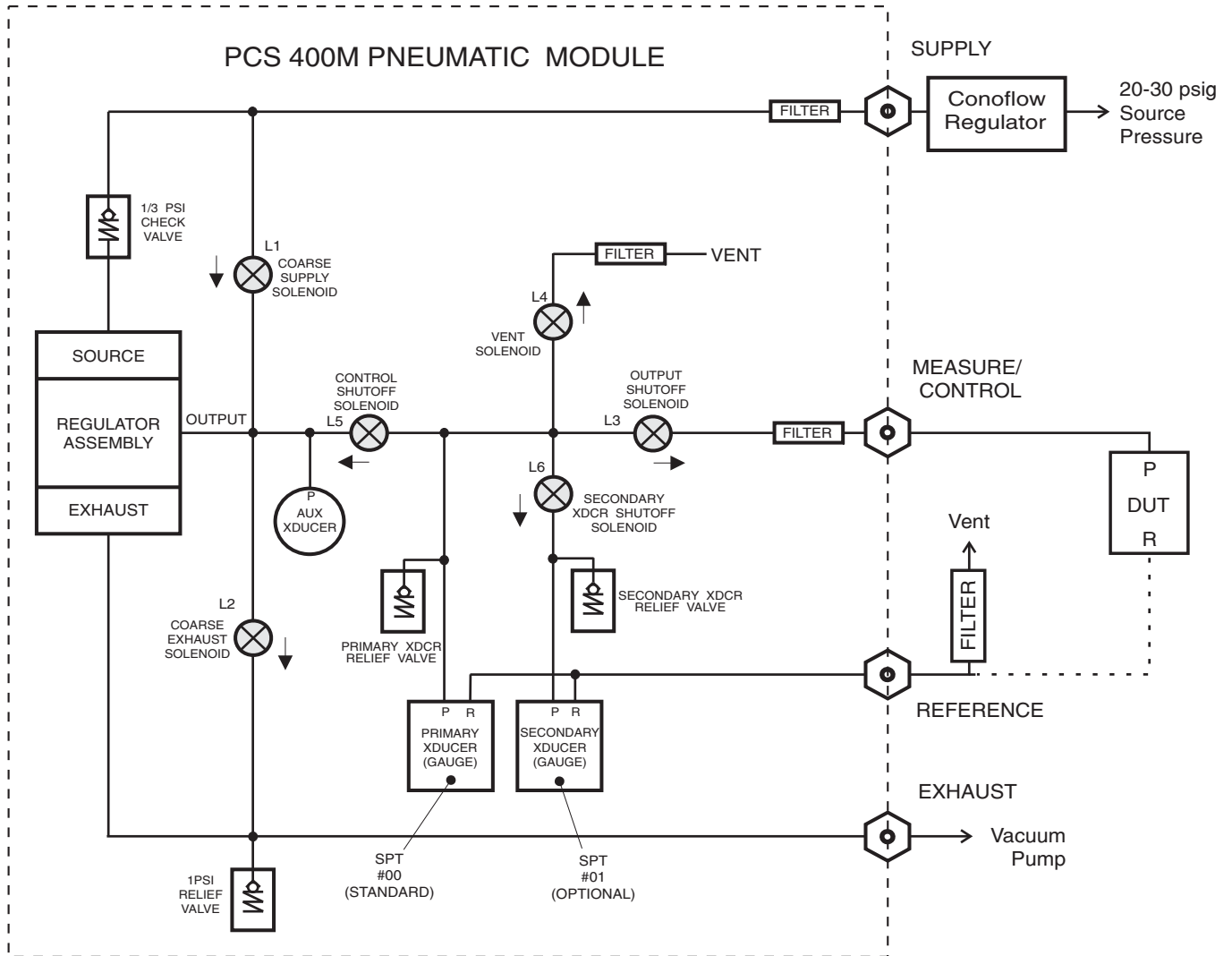
Figure 8.6 - Pneumatic Module for Low Pressure
