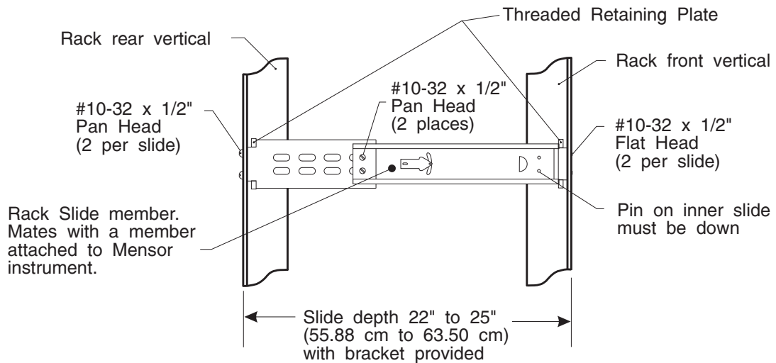
Figure 8.3 - Slide Specifications
