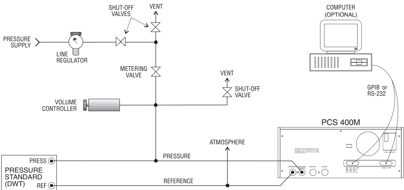
Figure 6.1 - Calibration Setup for Gauge Pressure
