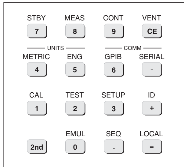
Figure 3.1 - Keypad
