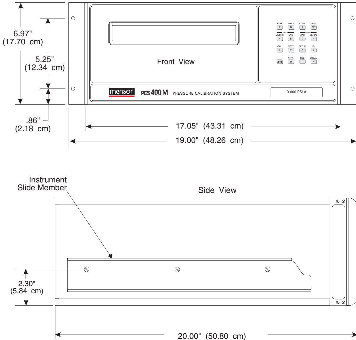
Figure 8.1 - Rack Mount Dimensions
