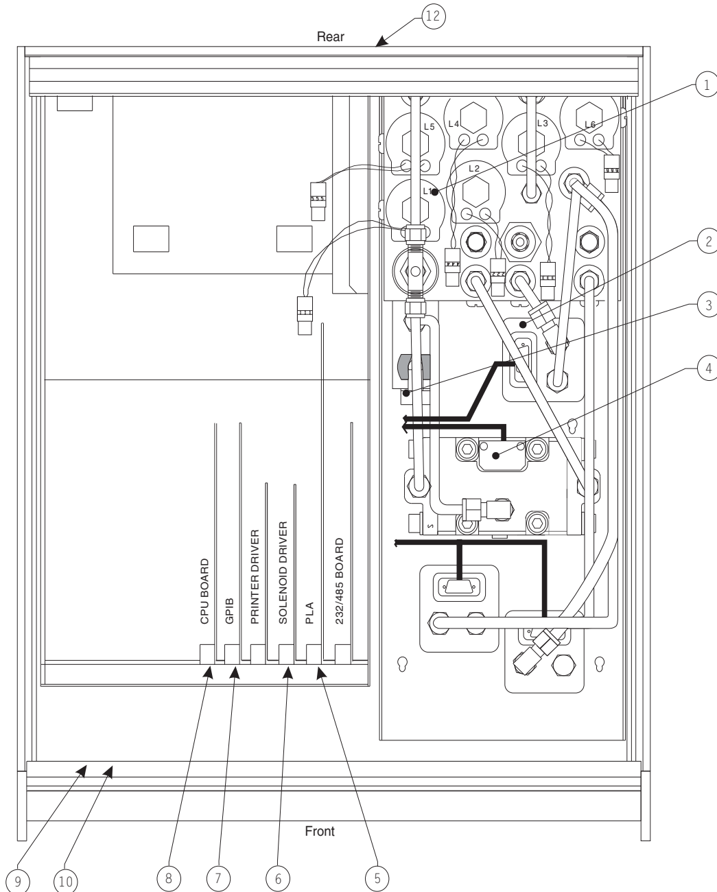
Figure 5.1 - Chassis Assembly-Top View
