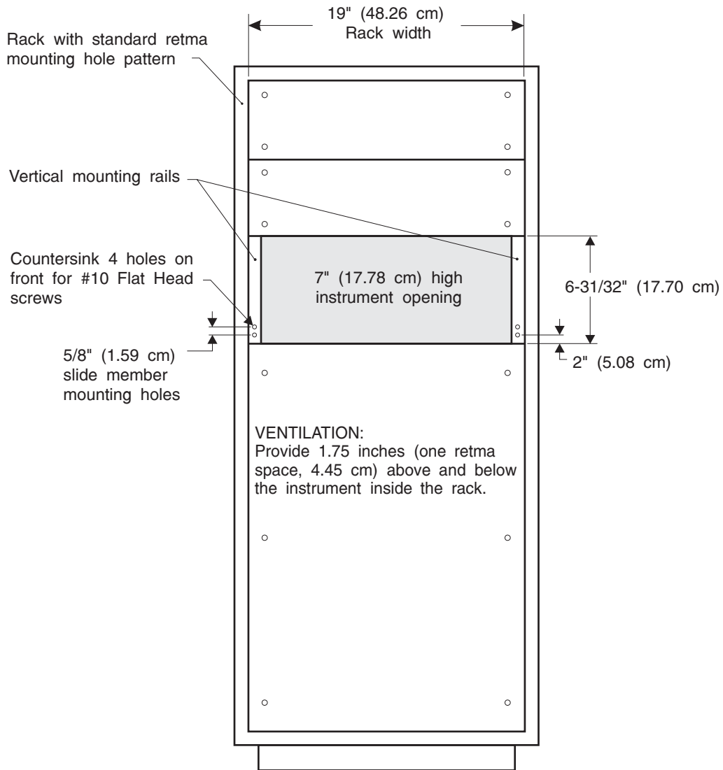
Figure 8.2 - Rack Specifications
