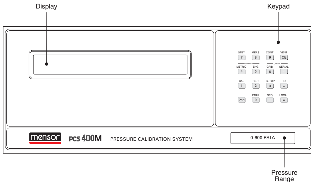
Figure 1.1 - Front Panel
