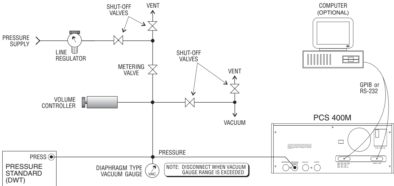
Figure 6.2 - Calibration Setup for Absolute Pressure
