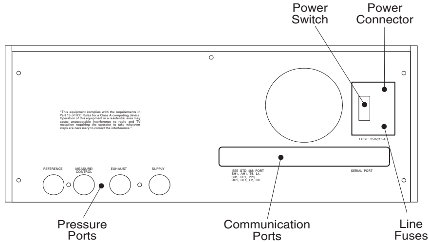
Figure 1.2 - Rear View
