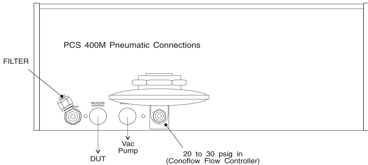
Figure 8.5 - Pneumatic Connections for Low Pressure
